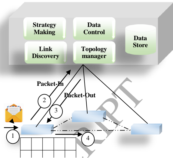
Figure 3: OpenFlow based flow
