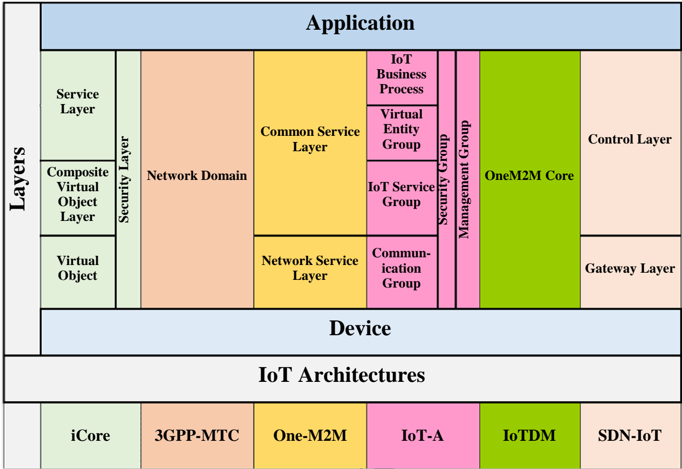
Figure 10: IoT Layered Architectures
