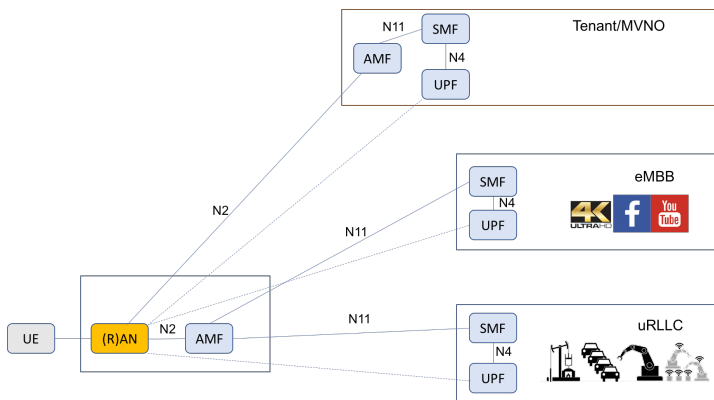
Figure 9: Example of AMF sharing among network slices.
