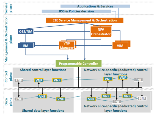
Figure 4: 5GPPP network orchestration architecture [99].
